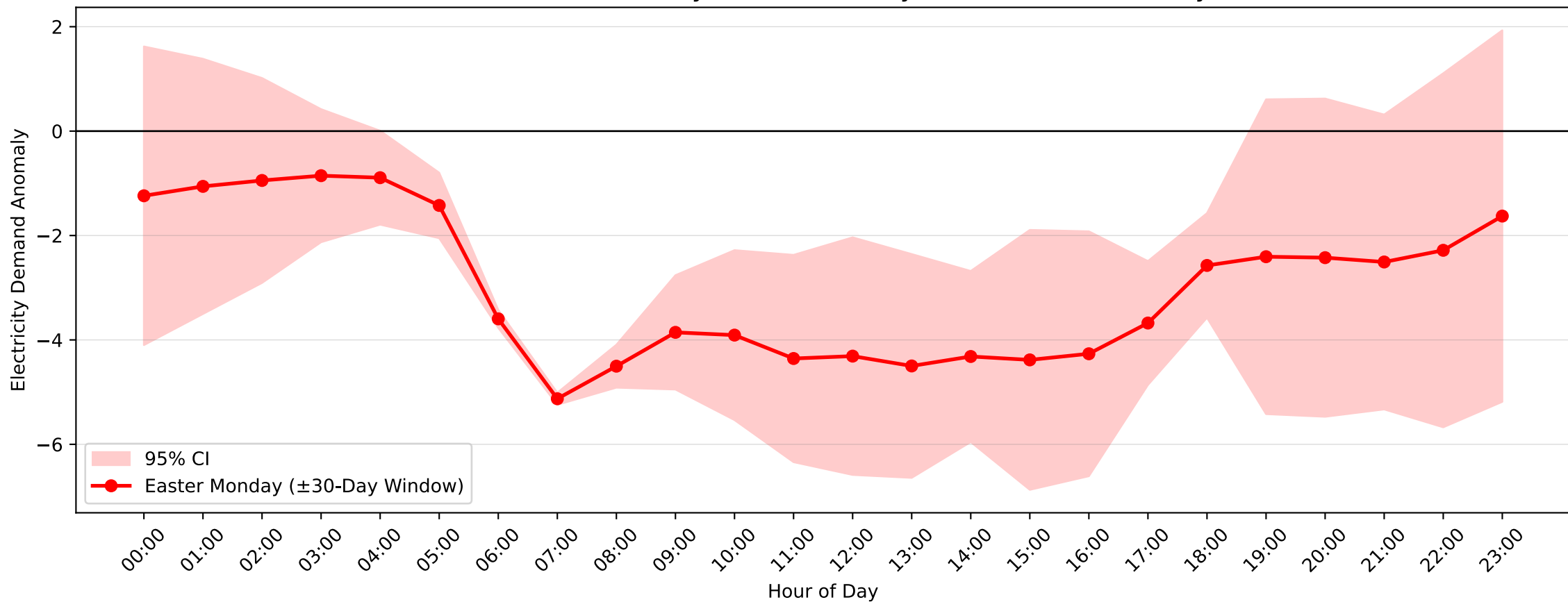
Hunters Hill Demand Anomaly: Easter Monday (2015–2016, \pm 30 -Day Window)
